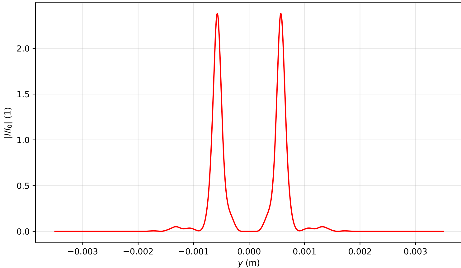
Intensity profile I(x=0, y, z=0.955)/I_0 , \text{Pin}=9.0\text{Pcr} , artificial time
